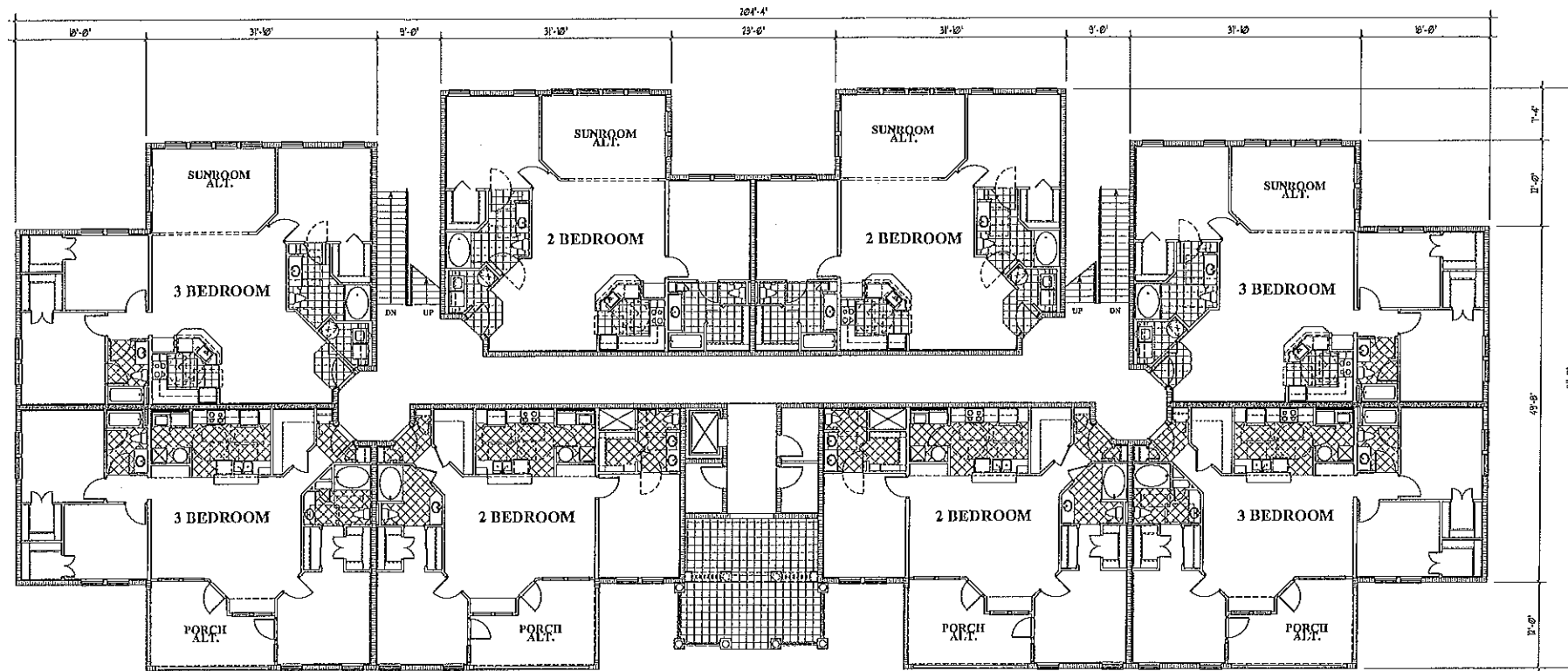
Second Level Floor Plan
