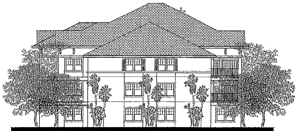
Side Elevation
