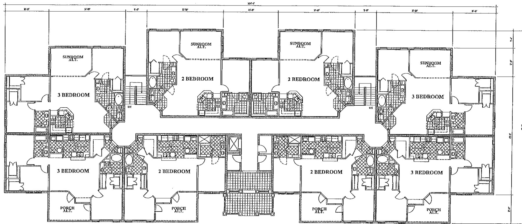
Fourth Level Floor Plan
