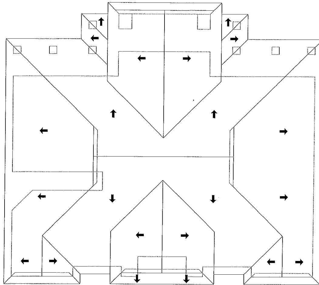
CLUBHOUSE ROOF PLAN
